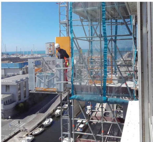
Material and passenger hoist Montacarichi materiali e persone PM - M10
