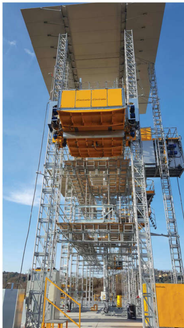
Material and passenger hoist Montacarichi materiali e persone ELSA PM-M50
